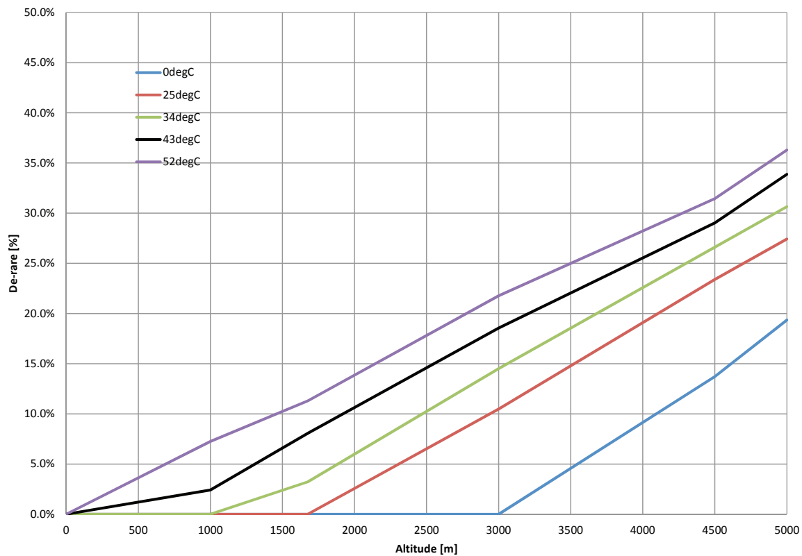
1106A-70TG1 50Hz Prime Power De-rate Chart
