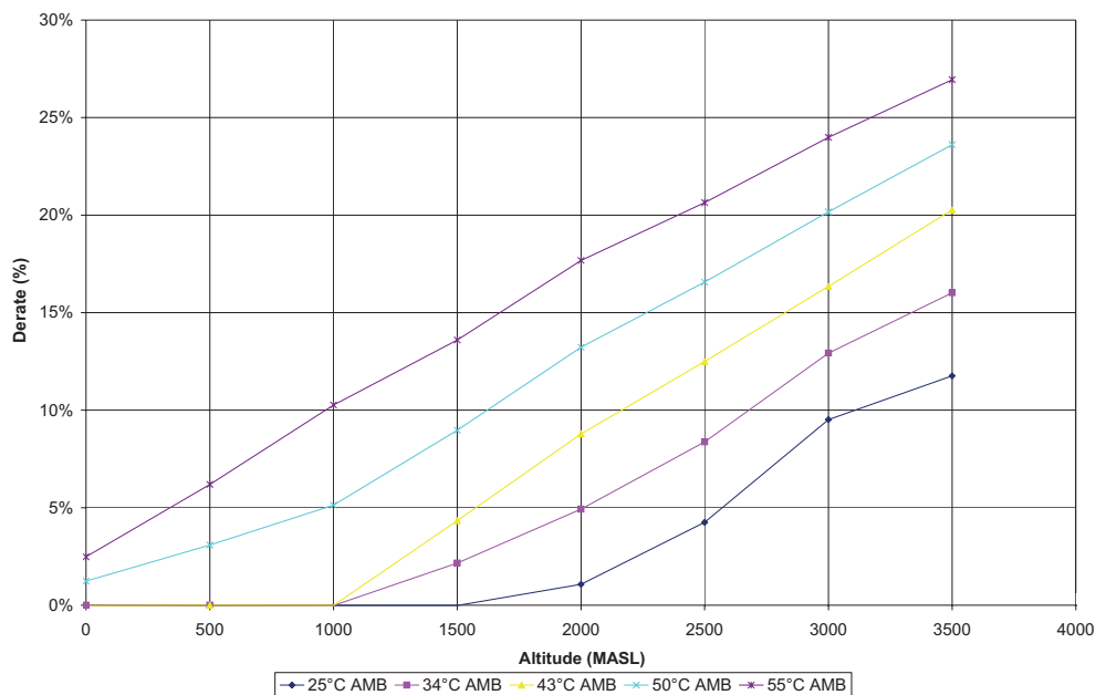
Derate Chart 2206A-E13TAG3 450 kVA Low BSFC
