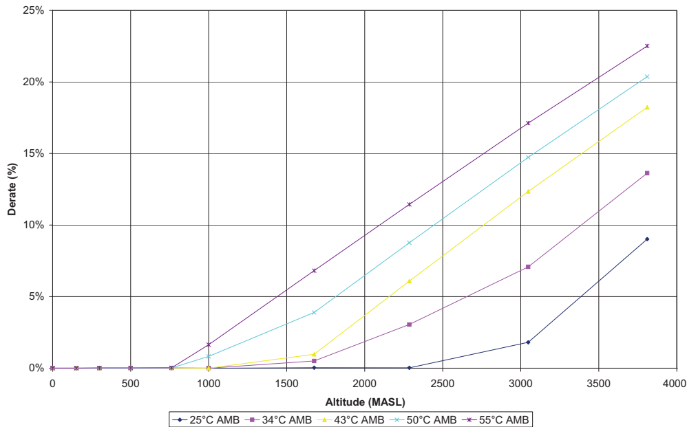
Derate Chart 2206A-E13TAG2 400 kVA Low BSFC
