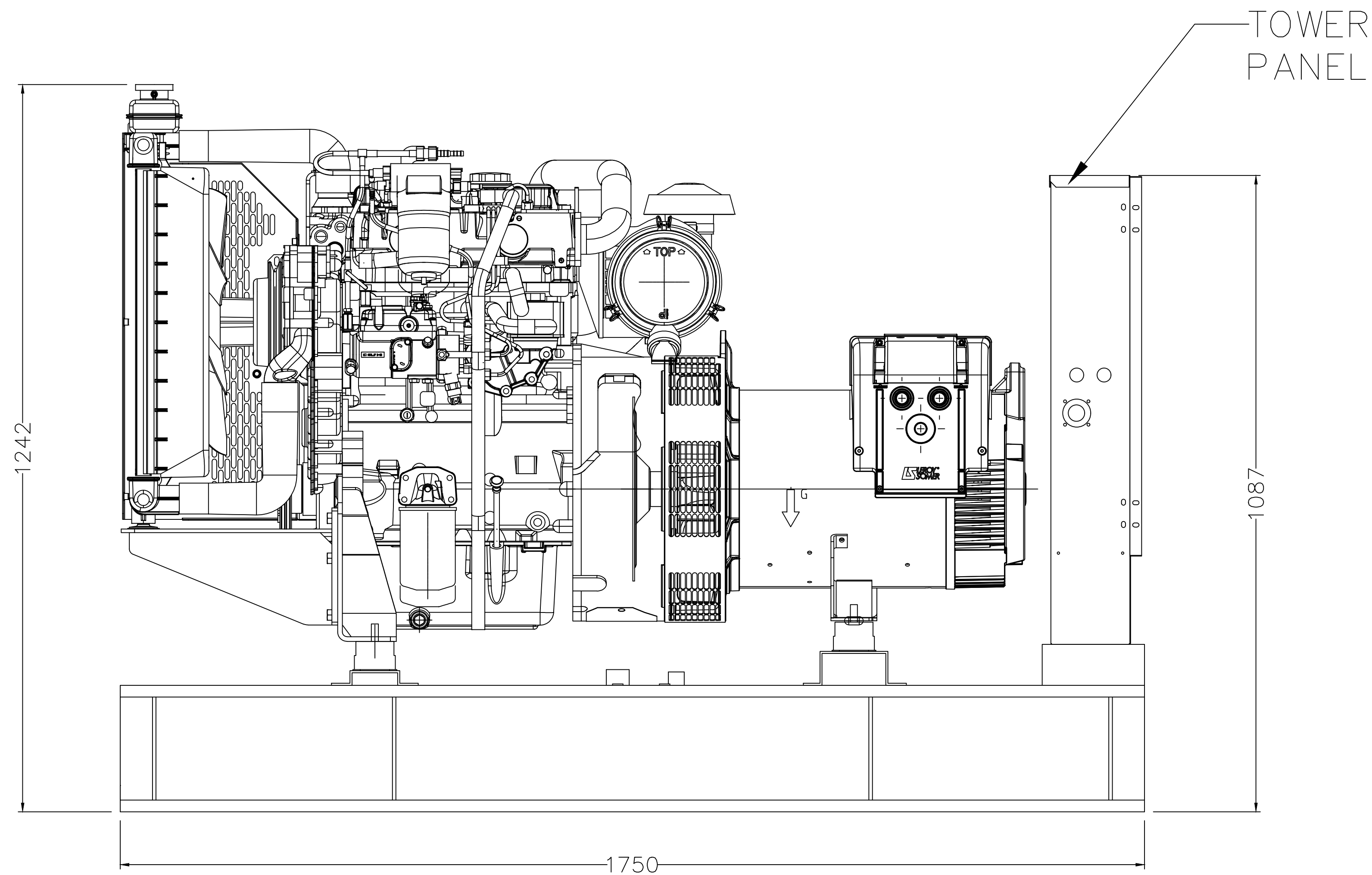
LEFT SIDE VIEW
