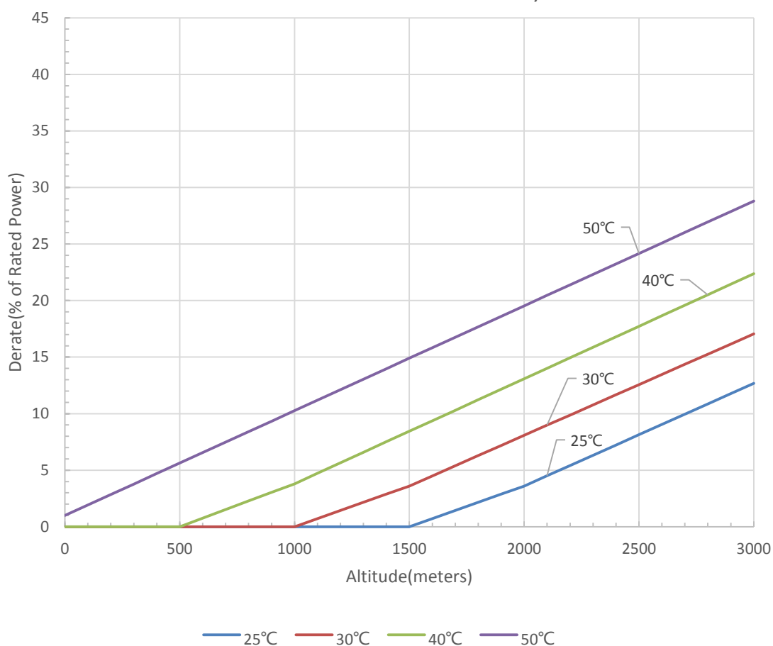
Derate Curves (Prime Power)
