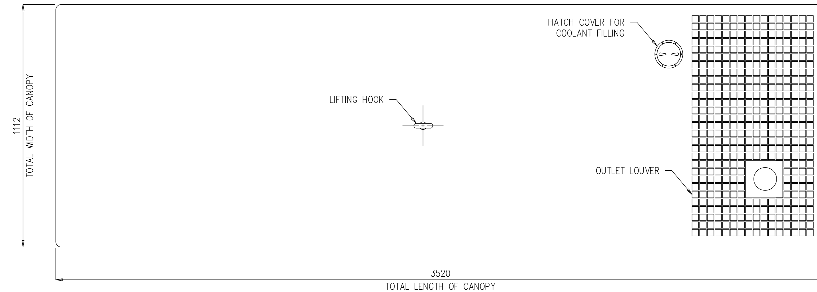
TOP VIEW
