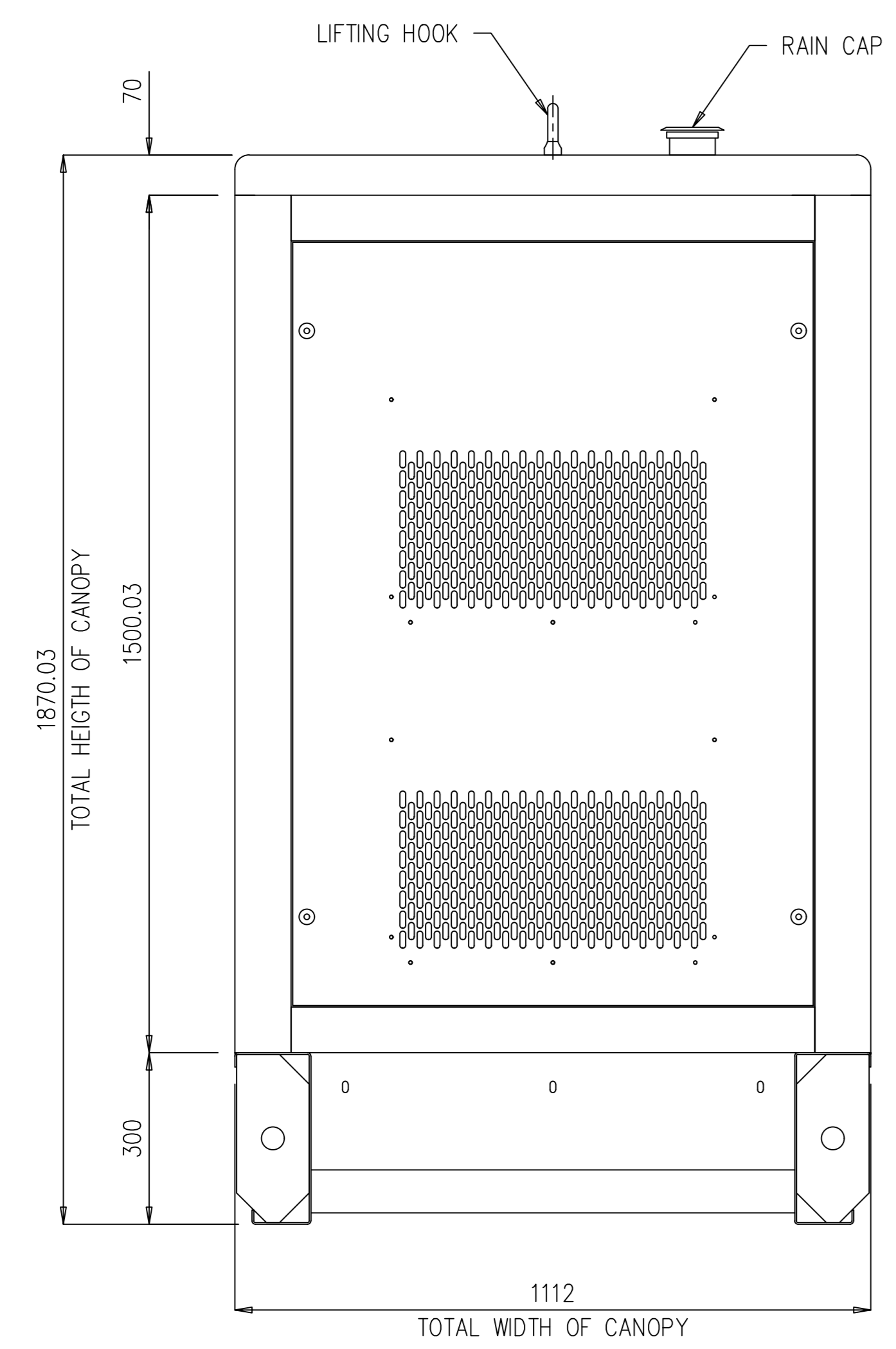
ALTERNATOR SIDE
