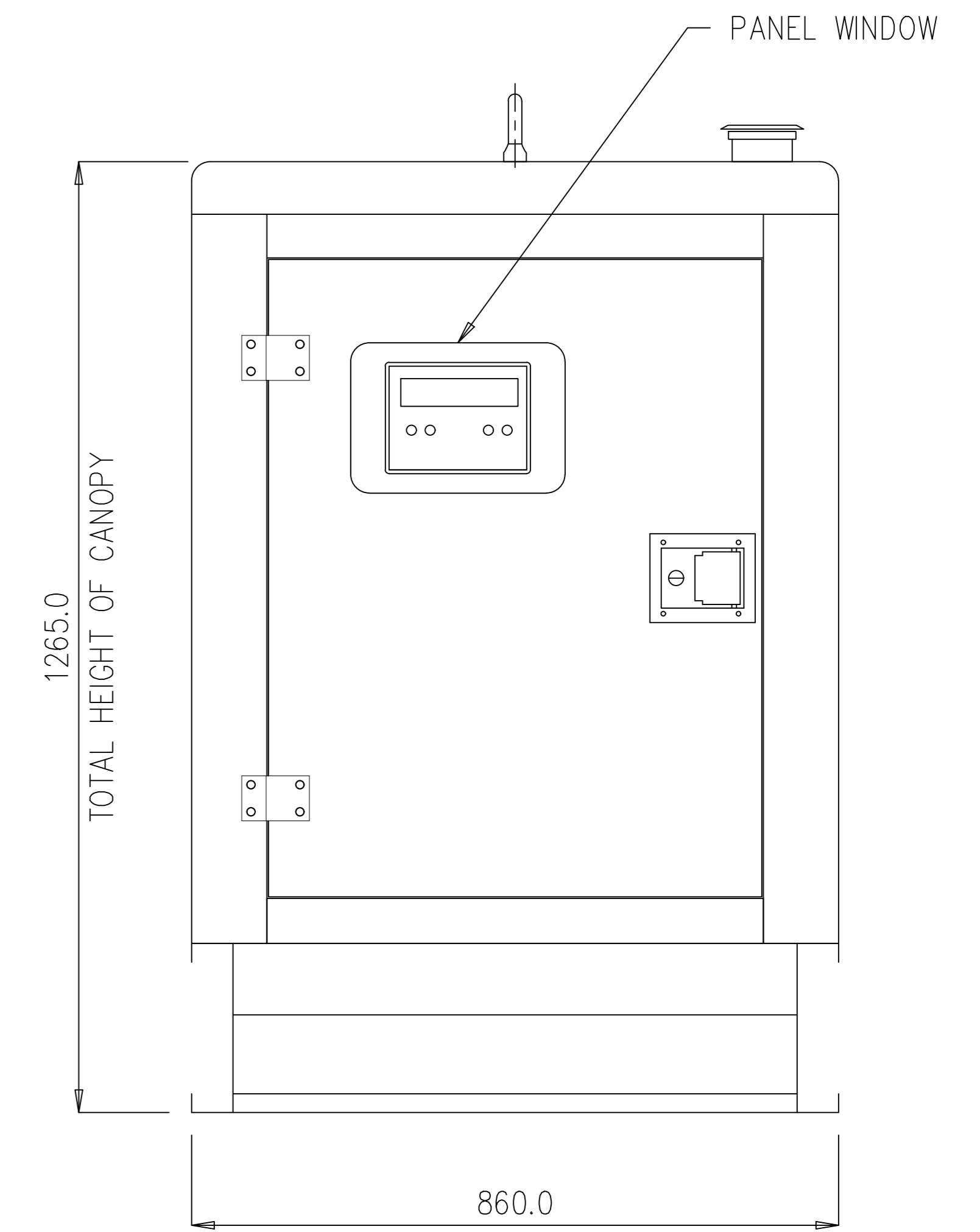
TOTAL WIDTH OF CANOPY
