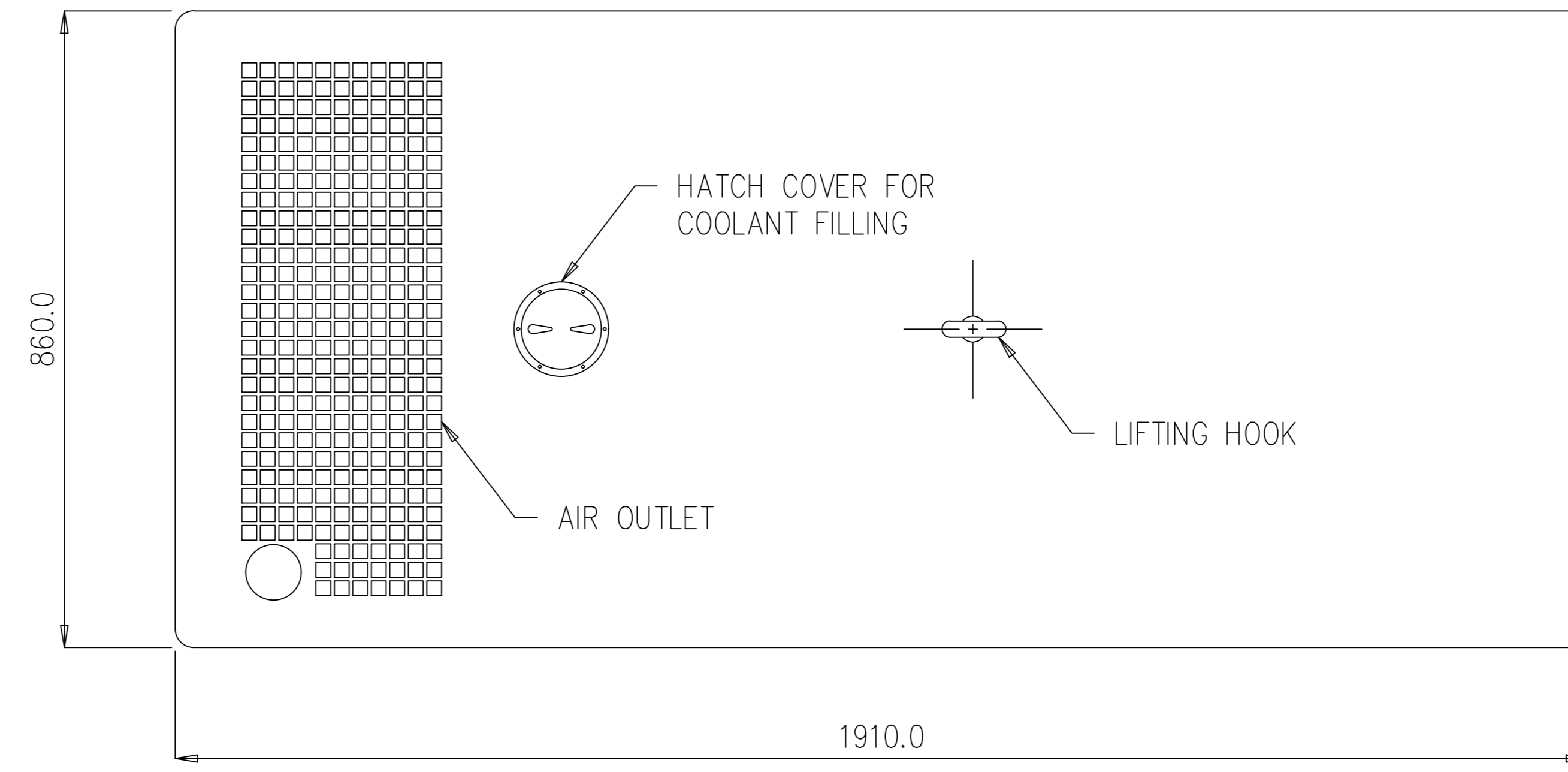
TOP VIEW
