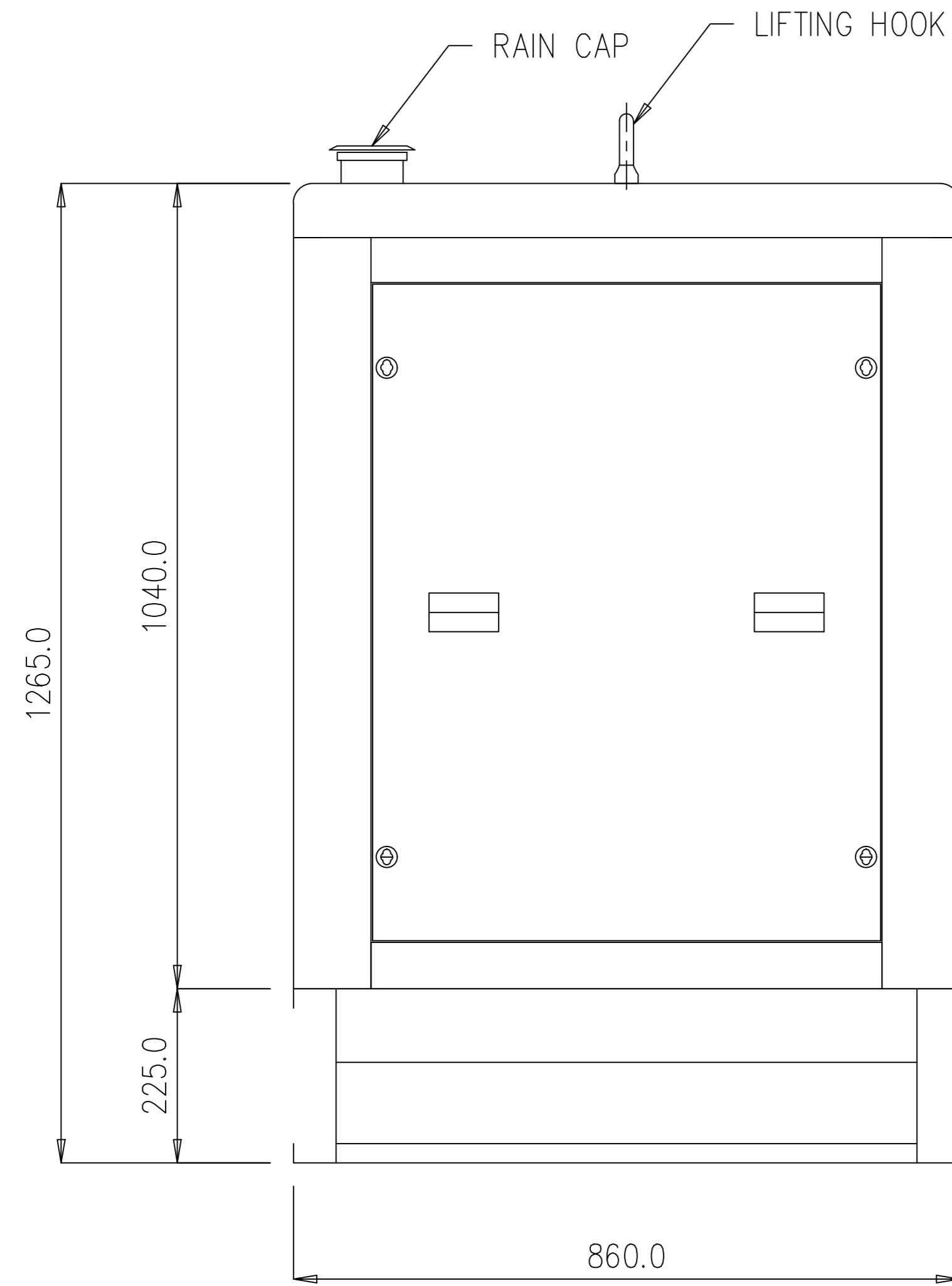
REAR VIEW
