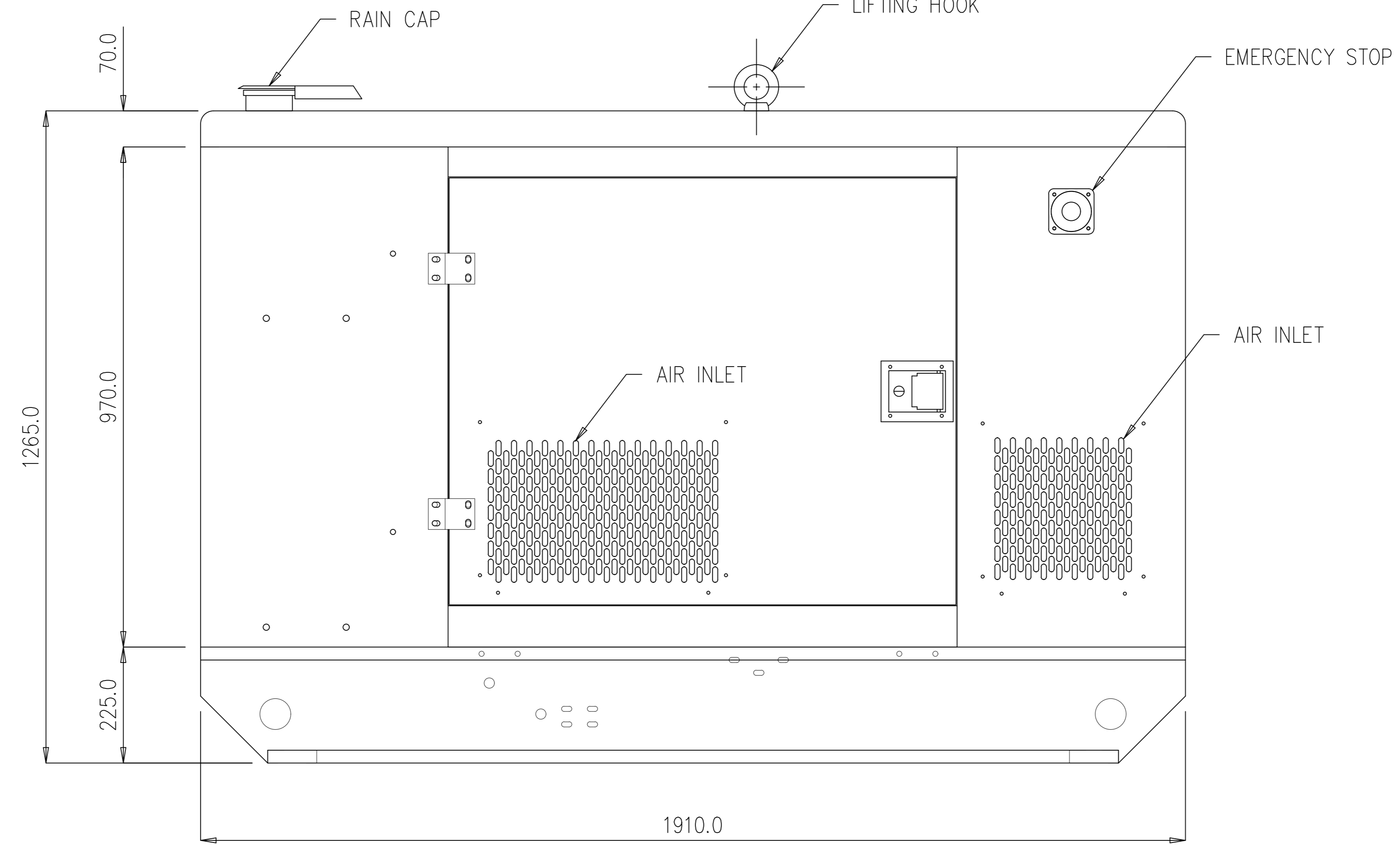
LEFT SIDE VIEW
