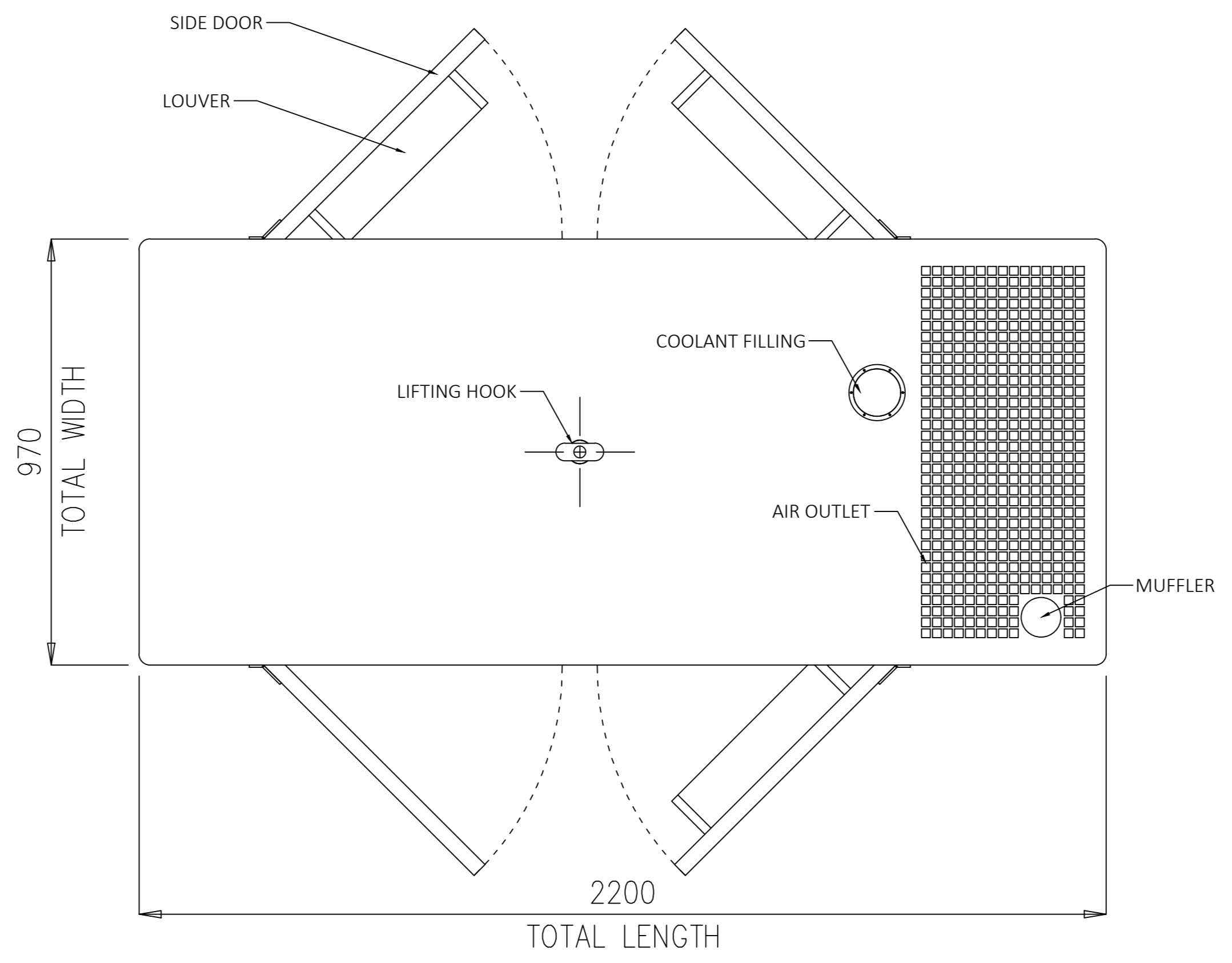
TOP VIEW
