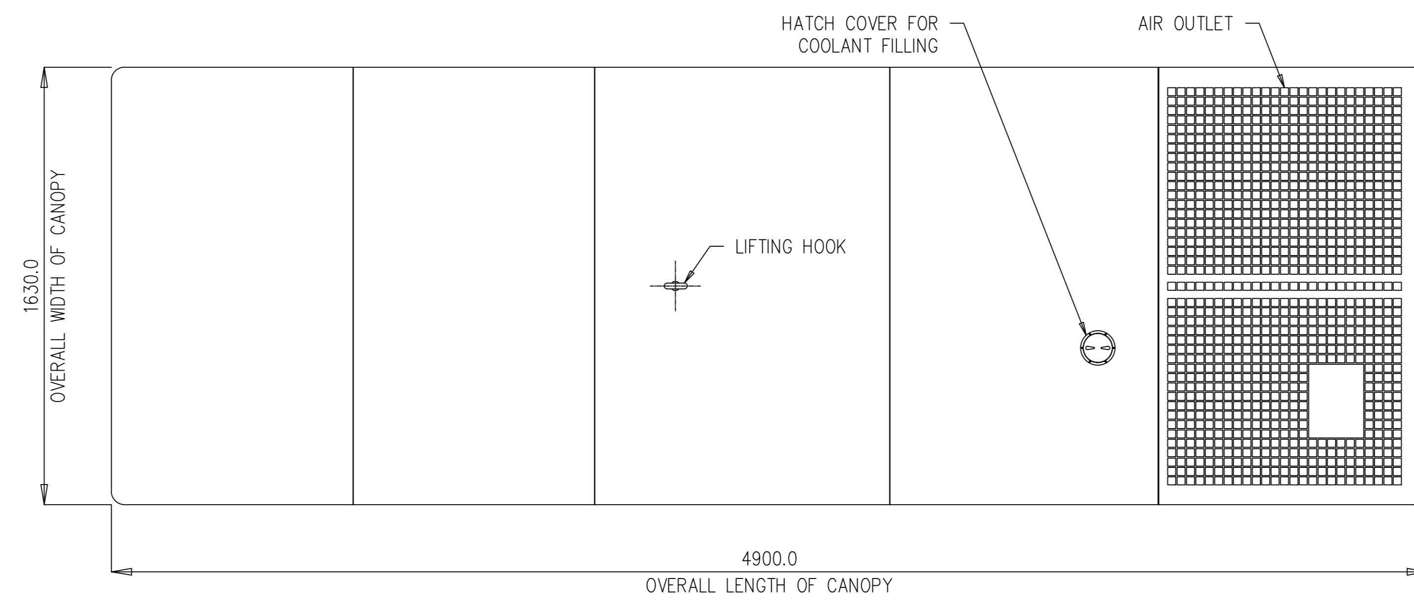
TOP VIEW
