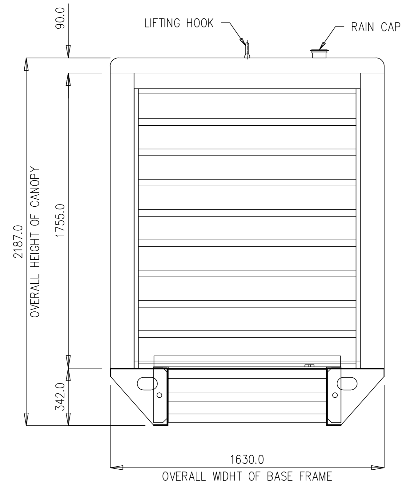
FRONT VIEW
