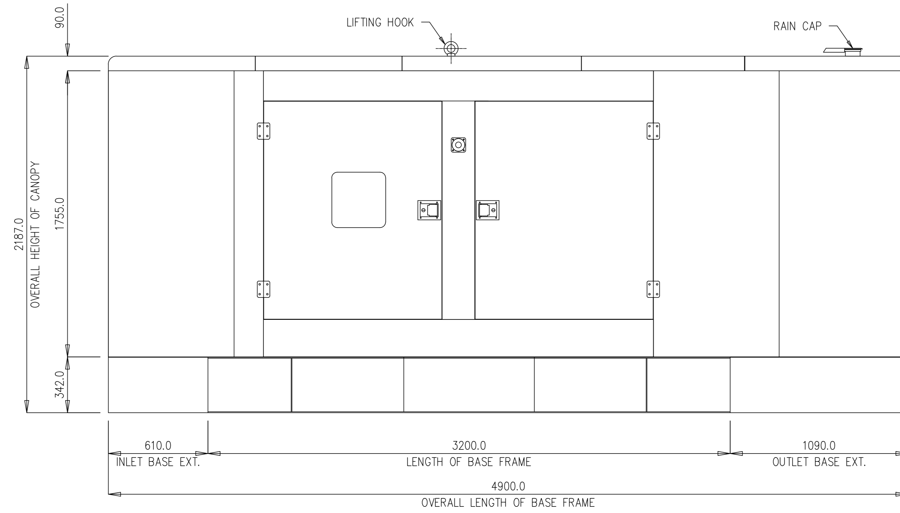
RIGHT SIDE VIEW
