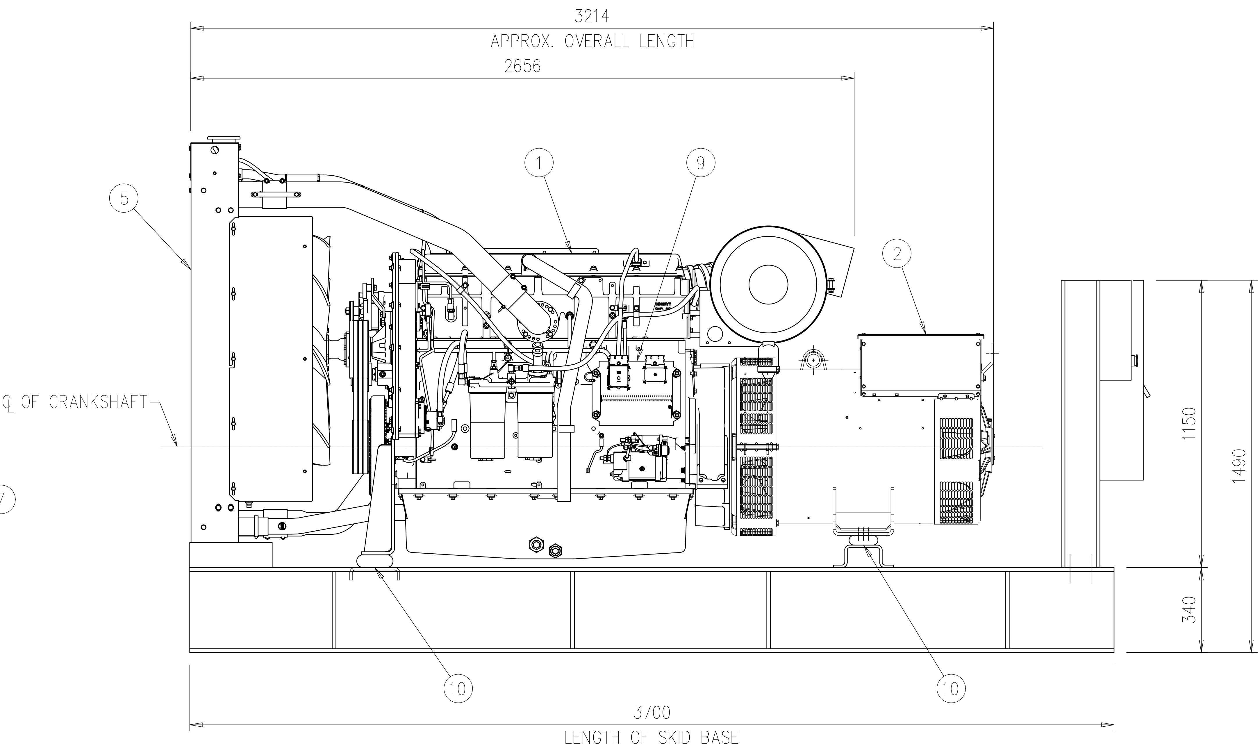
SIDE VIEW
