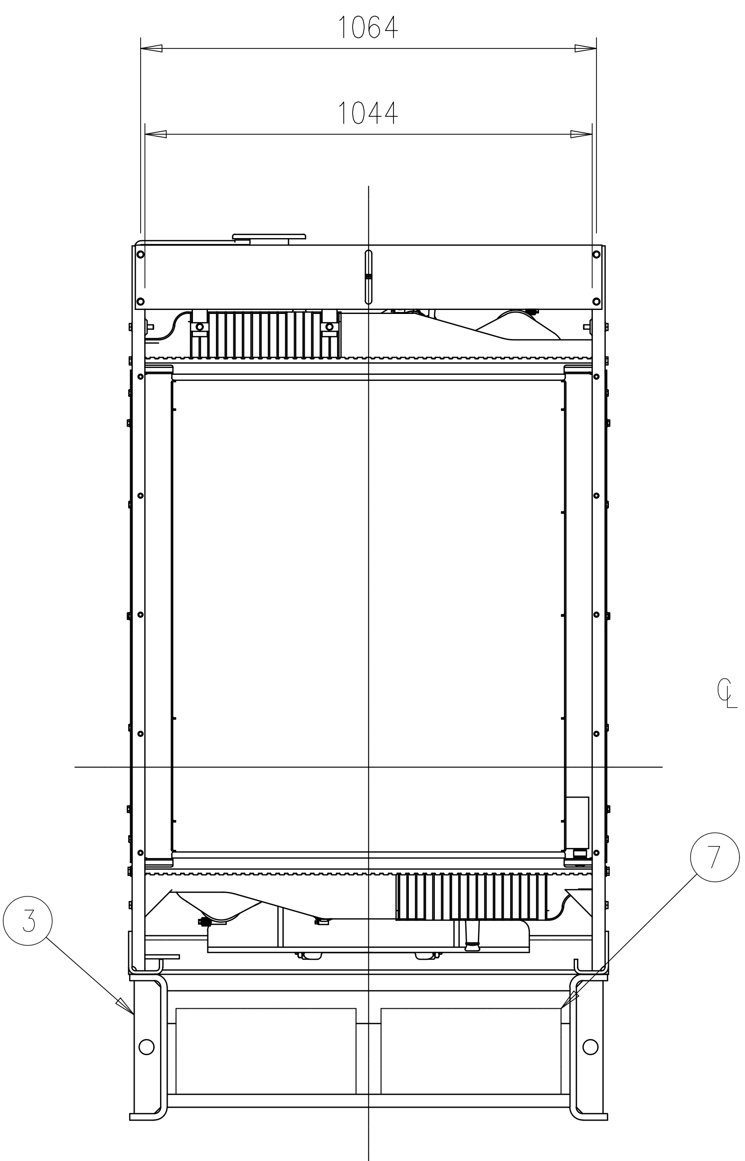
REAR VIEW
