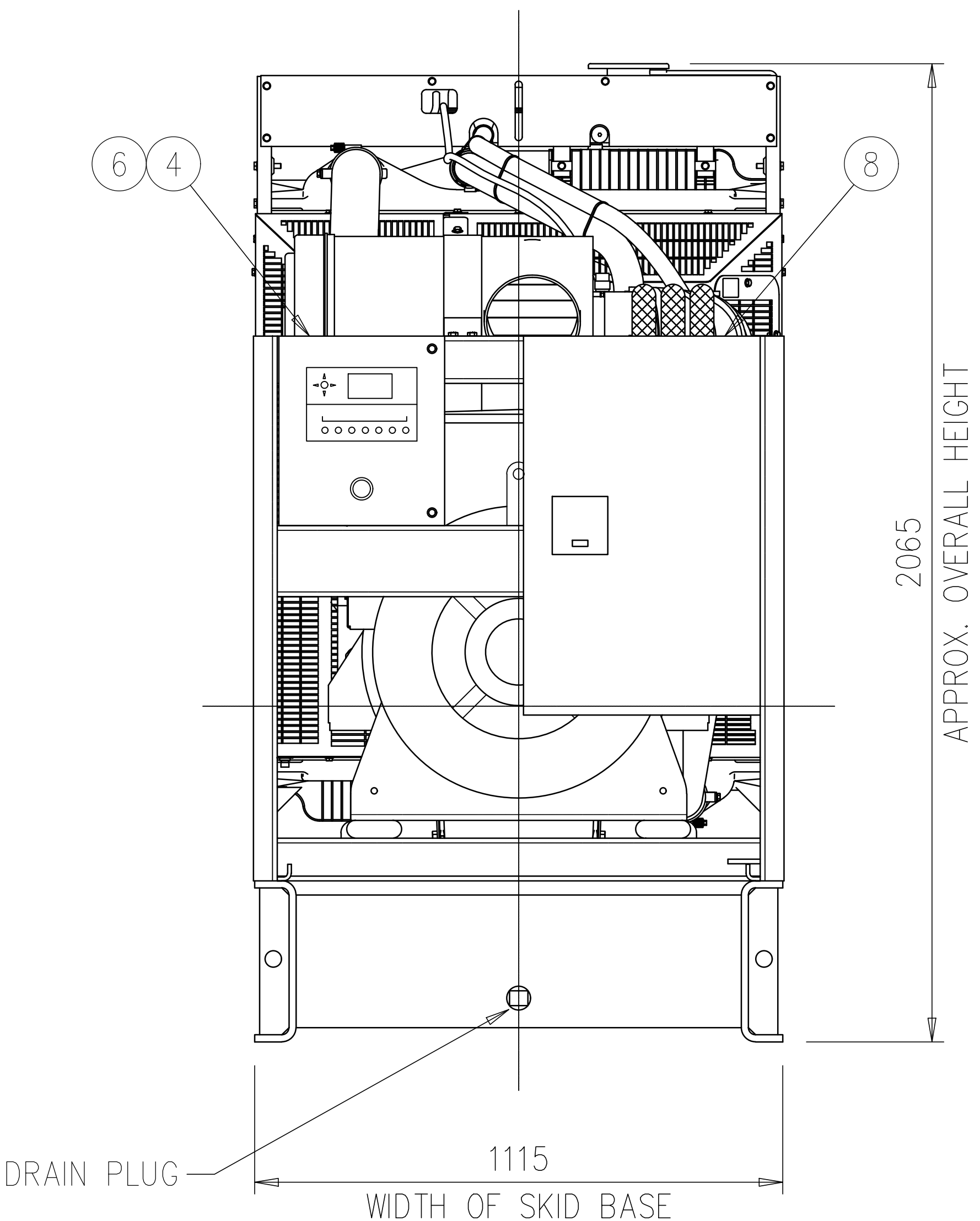
FRONT VIEW
