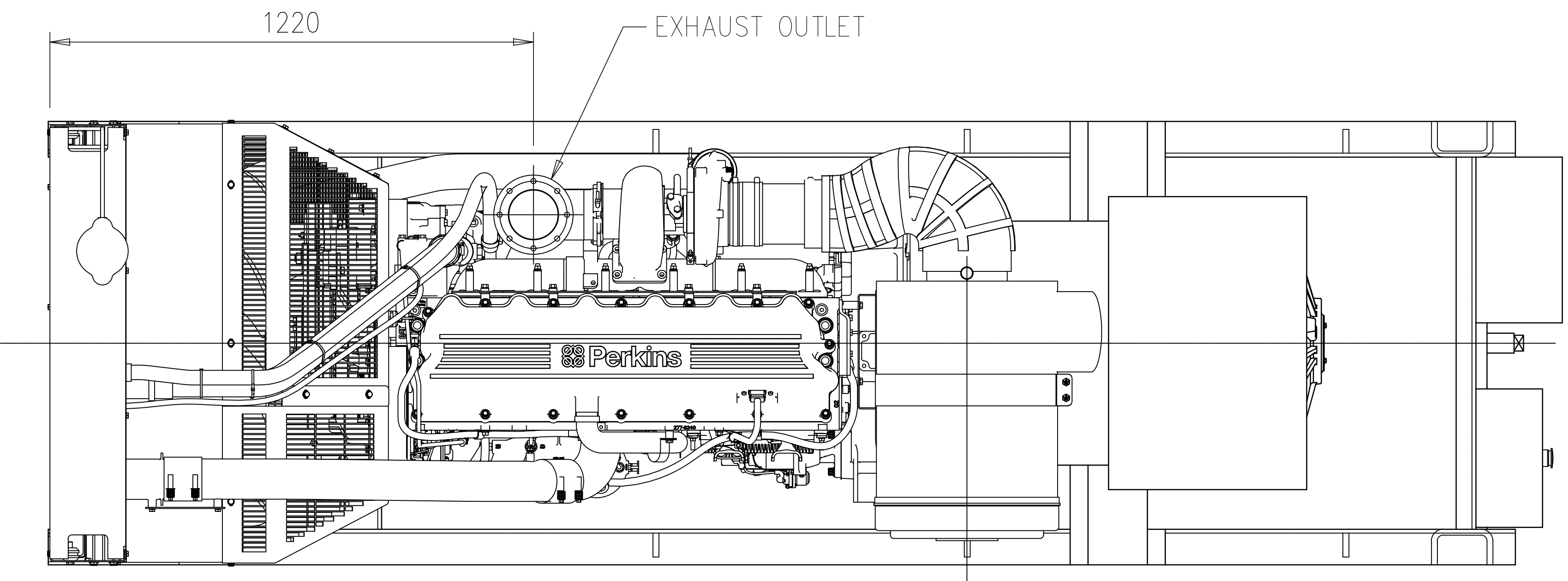
TOP VIEW
