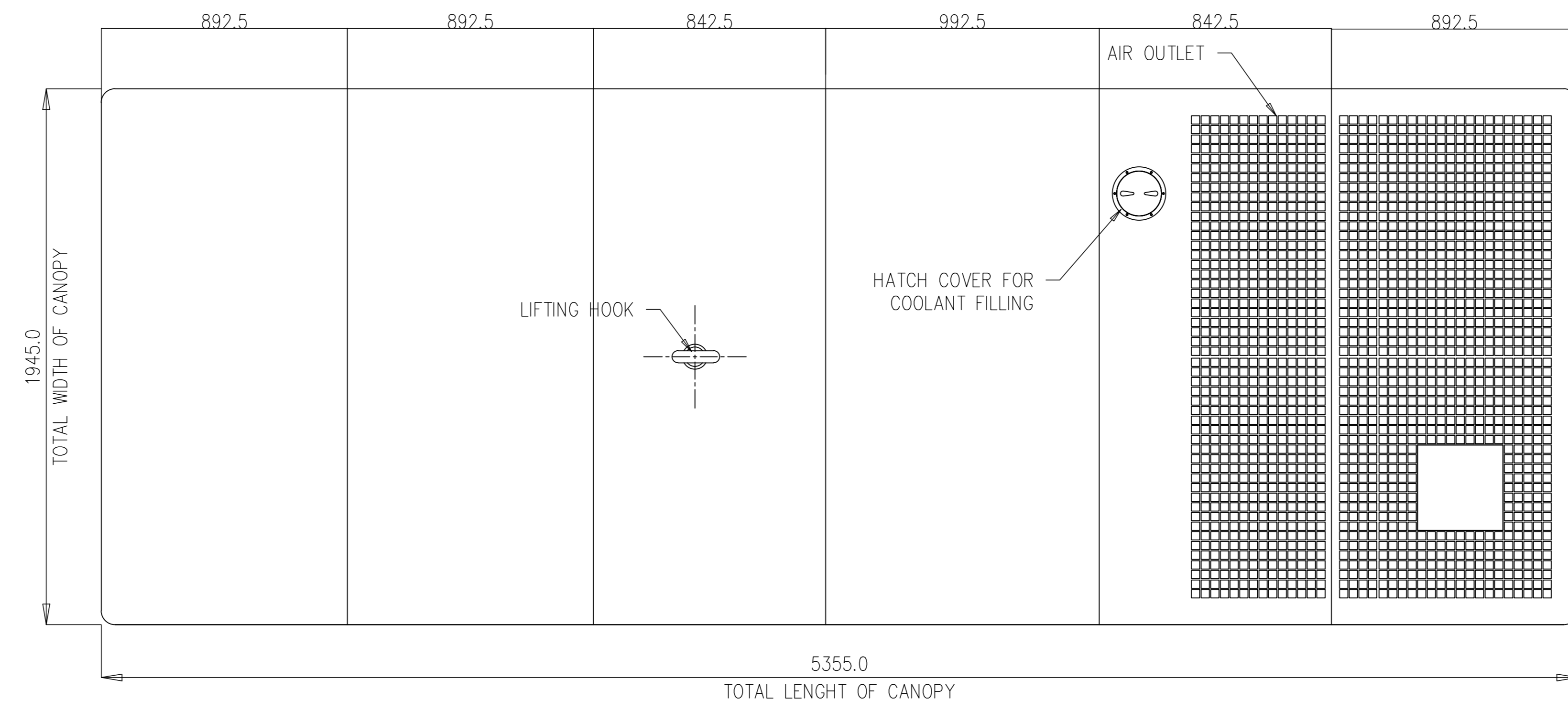
TOP VIEW
